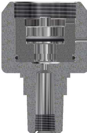
#2/3 7/8" SENSING UNIT
