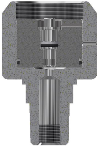
#4/5 3/8" SENSING UNIT
